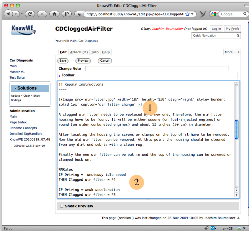
Fig. 9 Inline knowledge markup in KnowWE: (1) Inclusion of multimedia and (2) definition of derivation rules for the solution Clogged air filter.
