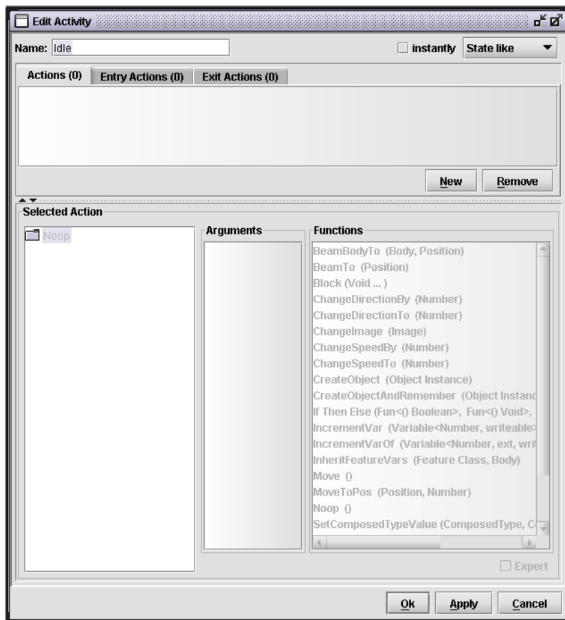
Figure 8: Operators on the activity reasoning engine editor
